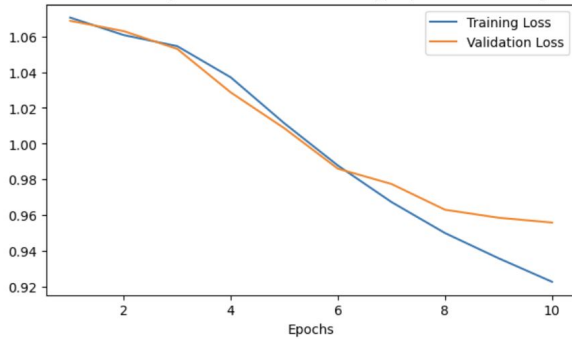
Loss for simplified LSTM model after hyperparameter tuning
